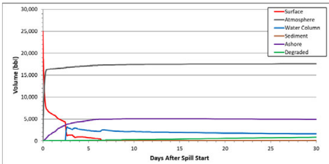
Figure 24: Amount of Oil in Different Environmental Compartments over Time: Cossackie–25,000 bbl Home Heating Oil–Summer–High Tide
