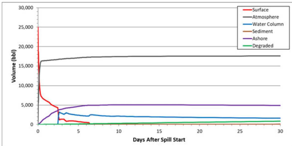
Figure 65: Percent Oil in Different Environmental Compartments over Time: Cocksackie–25,000 bbl Home Heating Oil–Summer–High Tide
