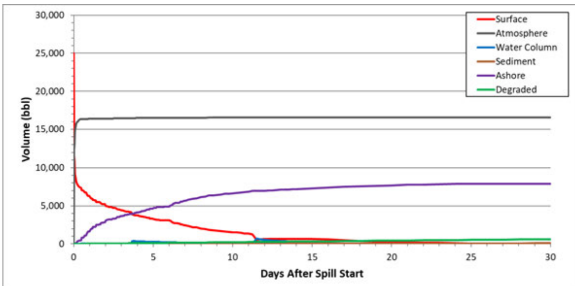
Figure 67: Percent Oil in Different Environmental Compartments over Time: Cocksackie–25,000 bbl Home Heating Oil–Winter–High Tide
