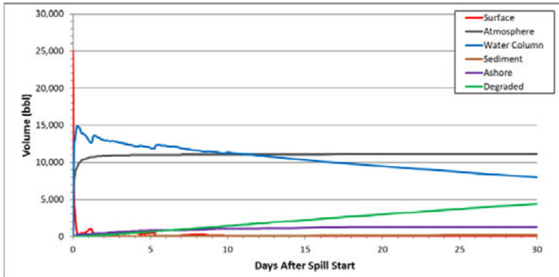
Figure 23: Amount of Oil in Different Environmental Compartments over Time: Cossackie–25,000 bbl Home Heating Oil–Spring–High Tide
