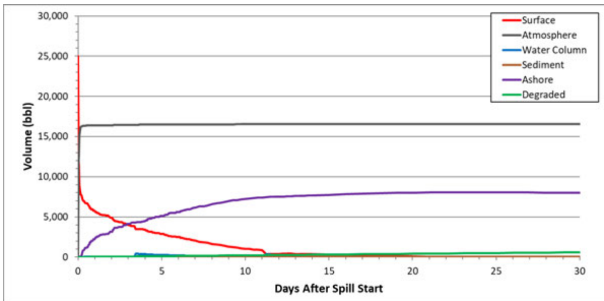
Figure 68: Percent Oil in Different Environmental Compartments over Time: Cocksackie–25,000 bbl Home Heating Oil–Winter–Low Tide
