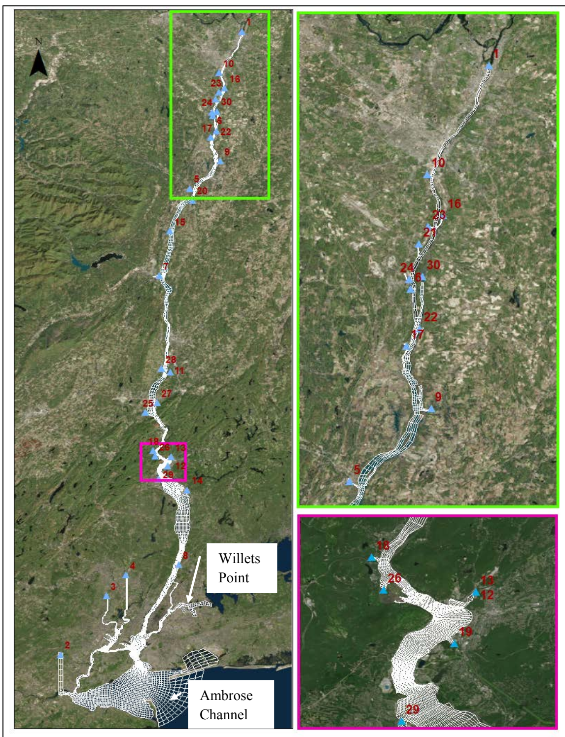
Figure 8: Model Grid and Forcing 16
